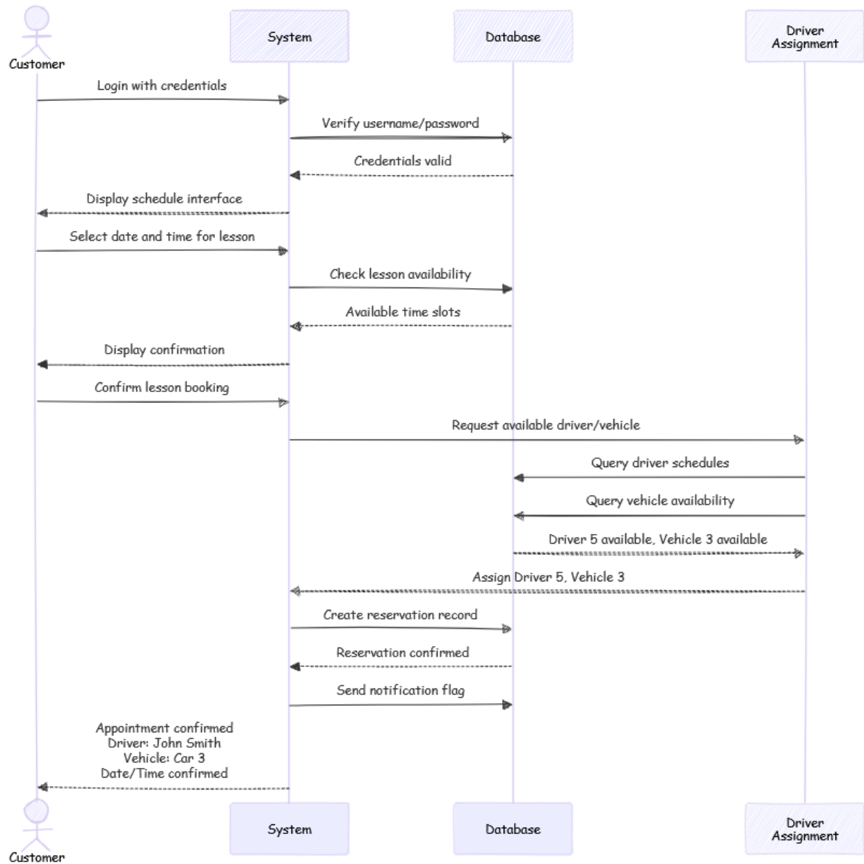
Figure 3: Sequence Diagram
